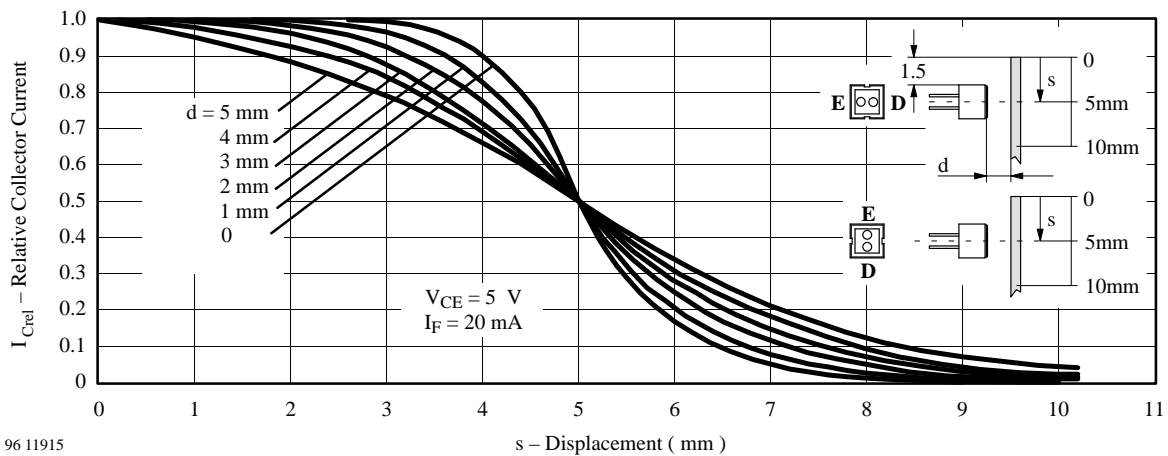
96 11915 Figure 11. Rel. Collector Current vs. Displacement
