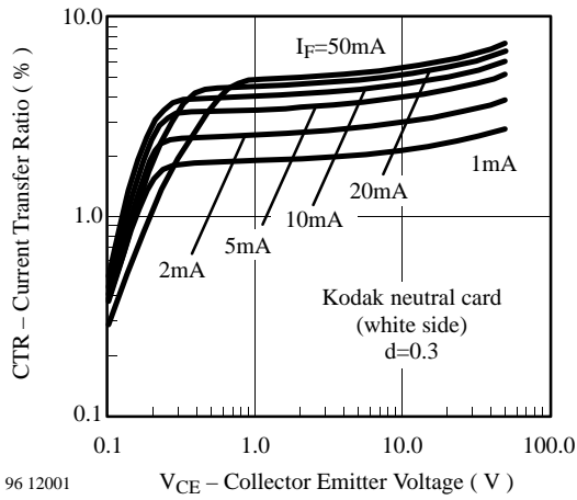
96 12001 Figure 8. Current Transfer Ratio vs. Collector Emitter Voltage
