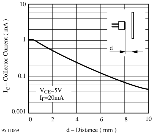
95 11069 Figure 9. Collector Current vs. Distance
