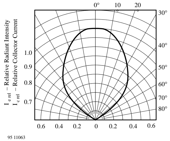
95 11063 Figure 10. Rel. Rad. Intensity/ Coll. Current vs. Displacement
